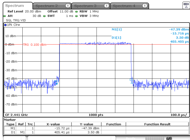
3DH1_Hopping
