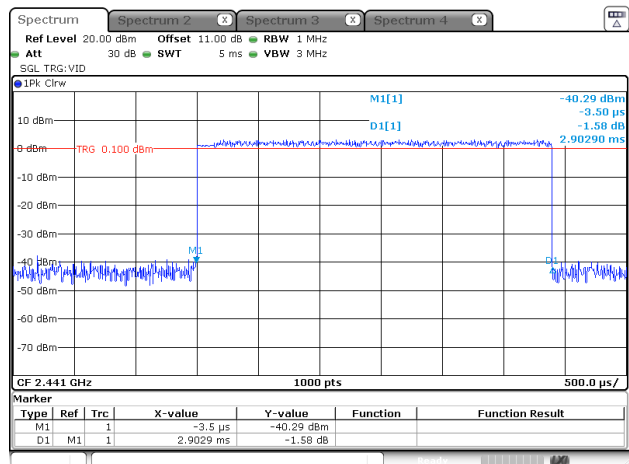
3DH5_Hopping
