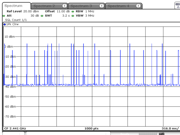
3DH5_Hopping
