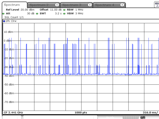
3DH3_Hopping
