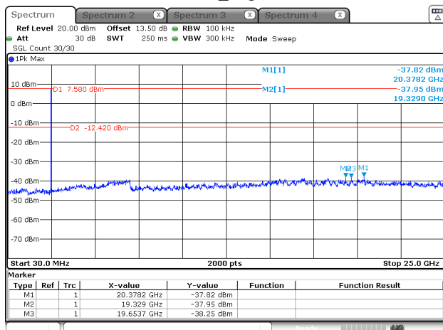
DH1_High
