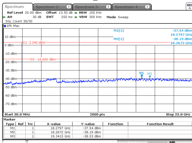
2DH1_Middle
