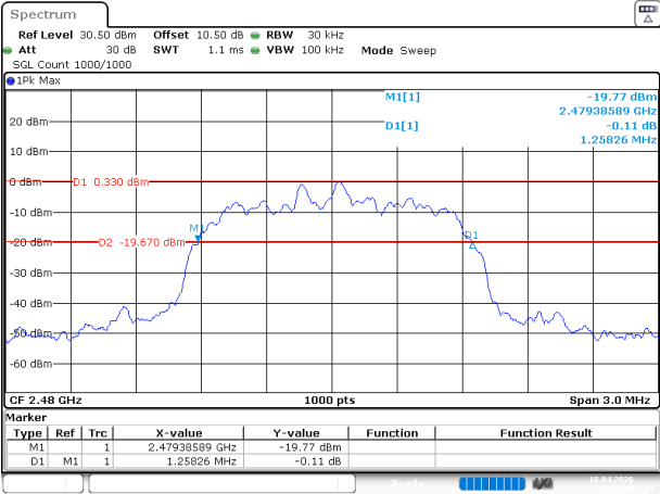
2DH1_High
