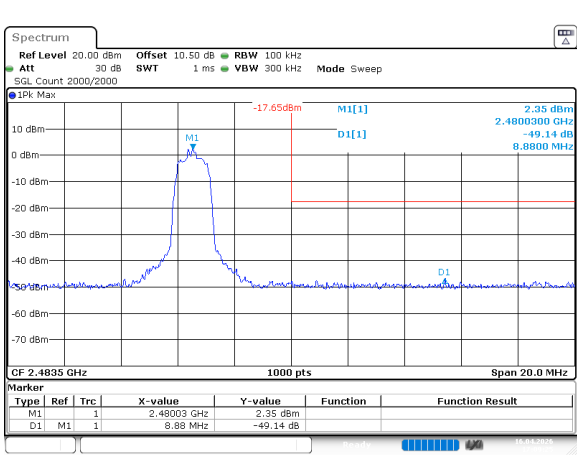
2DH1_High
