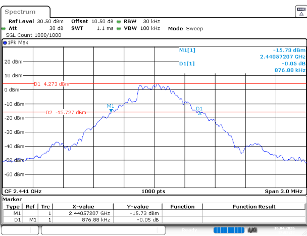
DH1_Middle
