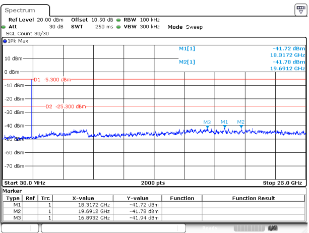
2DH1_Low
