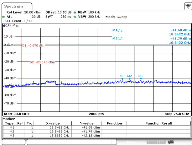
DH1_High
