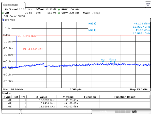
DH1_Low
