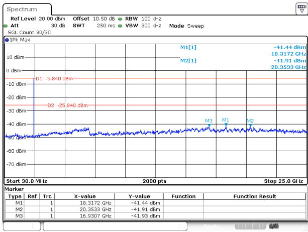
2DH1_Middle
