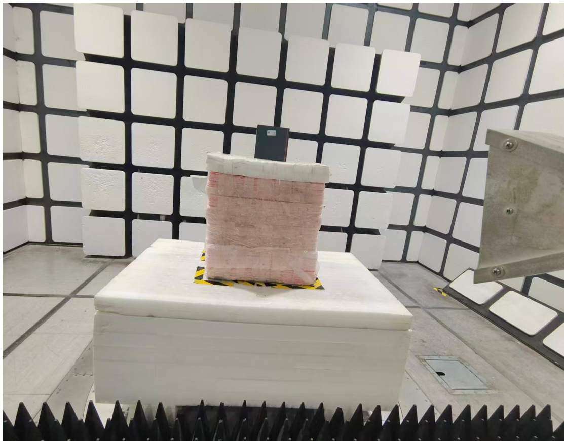
Radiated Emissions View (18-40 GHz)
