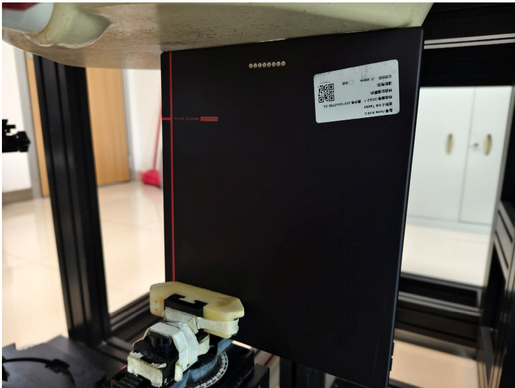
Body Bottom Setup Photo (0 mm)
