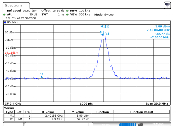
DH1_Low
