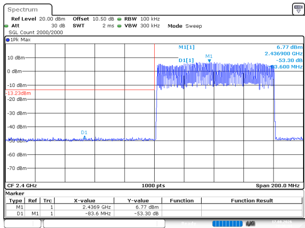
DH1_Hopping_Lower
