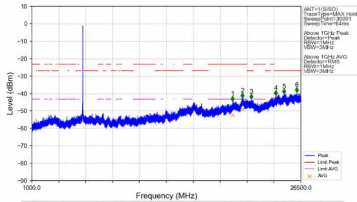
802.11a_HCH_5825MHz_Ant1_NTNV
