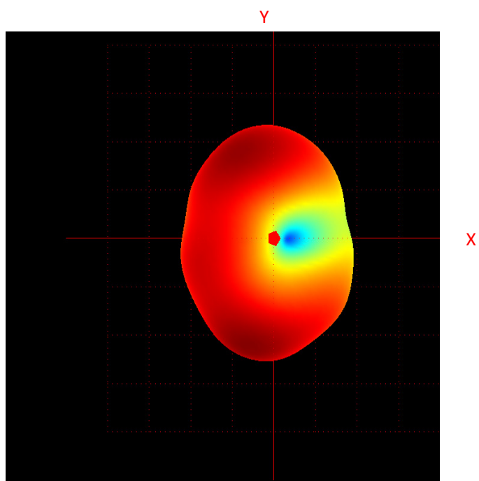
Direction map GSM850 WCDMA Band 5
