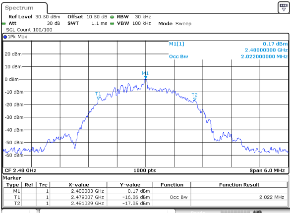
BLE_2M_High_Channel
