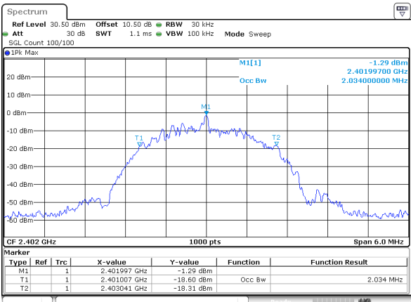
BLE_2M_Low_Channel
