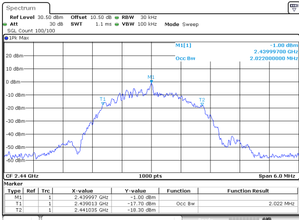
BLE_2M_Middle_Channel
