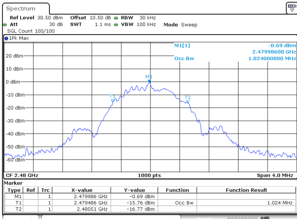
BLE_1M_High_Channel
