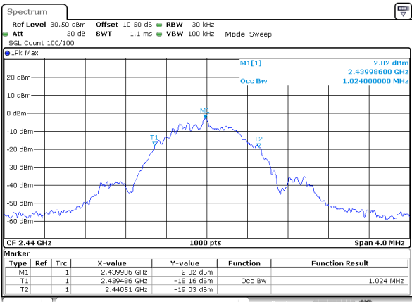
BLE_1M_Middle_Channel
