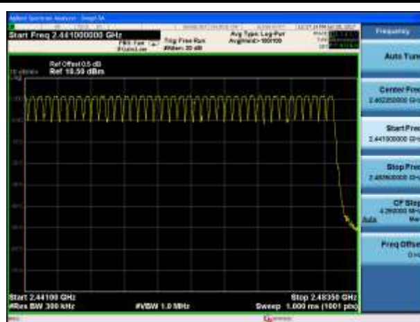
3-DH5(2Mbps)-2441~2483.5MHz
