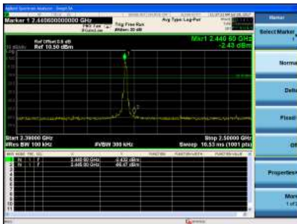
CH39 (2441MHz) 3-DH5(3Mbps)
