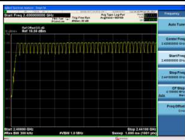
3-DH5(3Mbps)-2400~2441MHz
