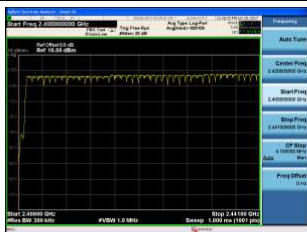
3-DH5(3Mbps)-2400~2441MHz
