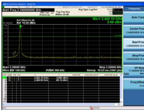
CH00 (2402MHz) DH5(1Mbps)
