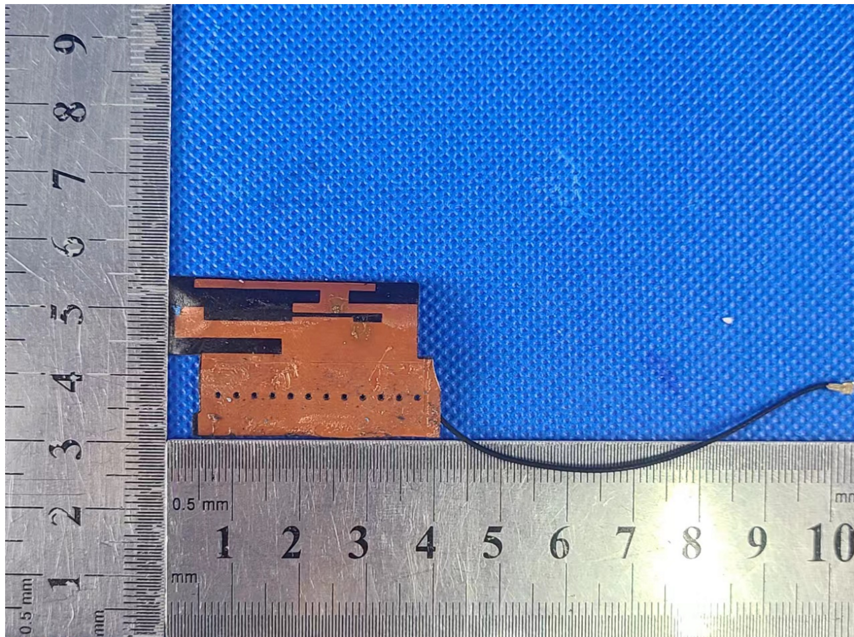
Antenna Photo
