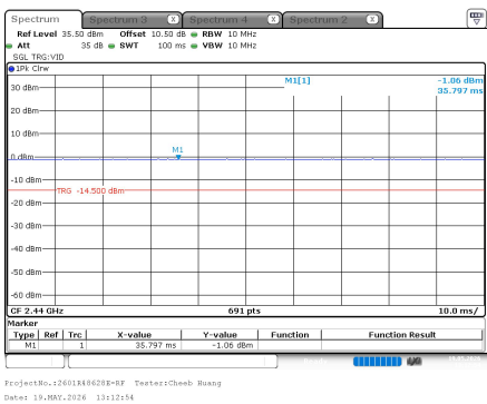
BLE_2M_Middle_Channel
