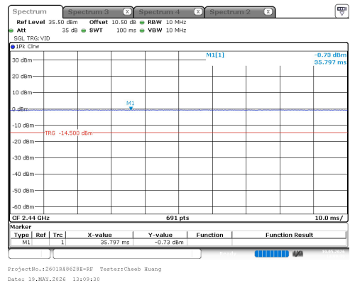
BLE_1M_Middle_Channel
