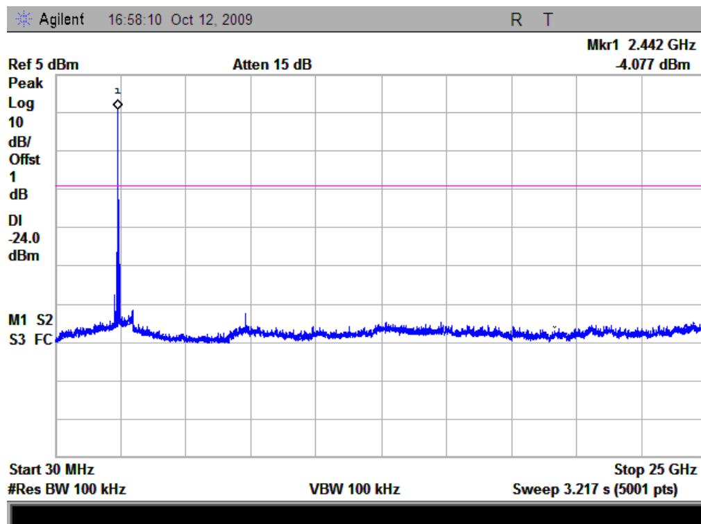
(Plot B: Channel = 39, 30MHz to 25GHz)
