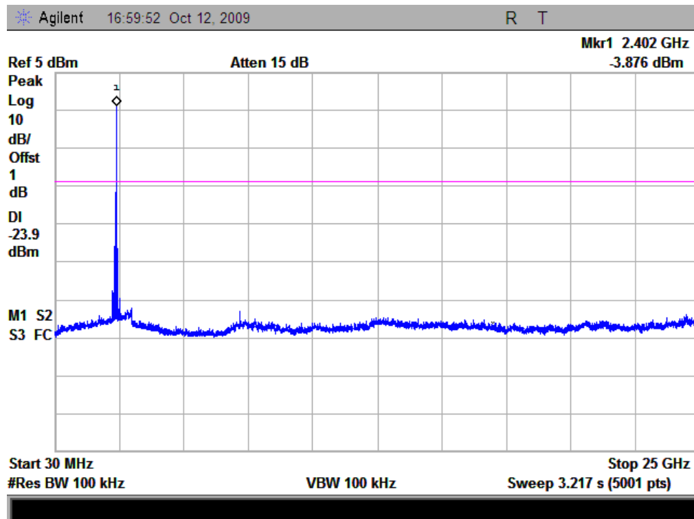
(Plot A: Channel = 0, 30MHz to 25GHz)
