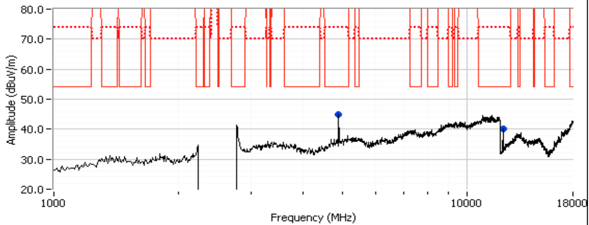
CH39, EUT Upright
