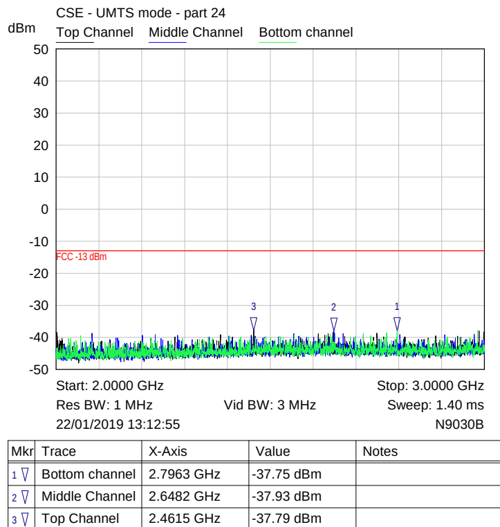
Plot of conducted emissions 2 GHz – 3 GHz range
