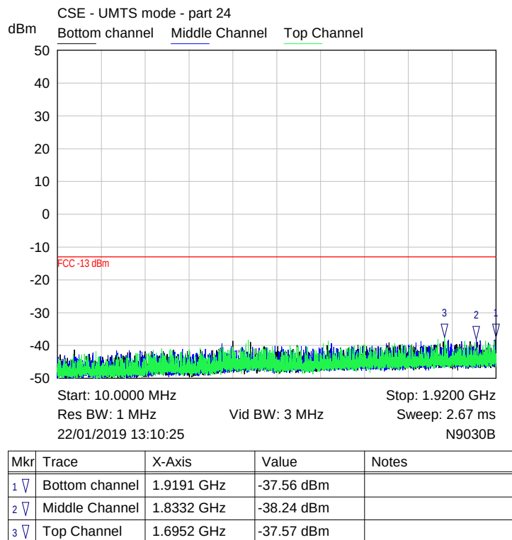
Plot of conducted emissions 10 MHz – 1920 MHz range
