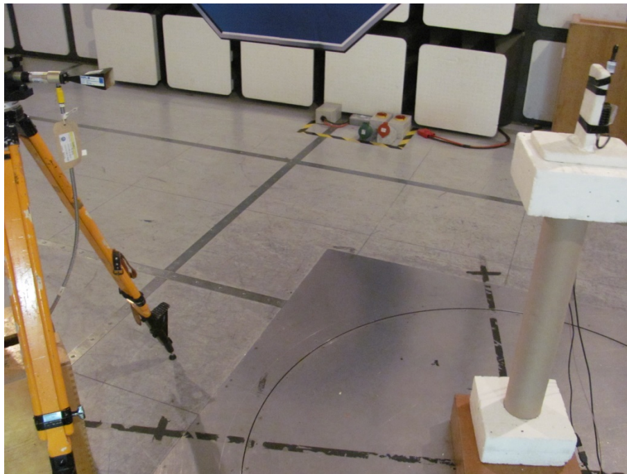
Radiated Emission 18 GHz to 25 GHz
