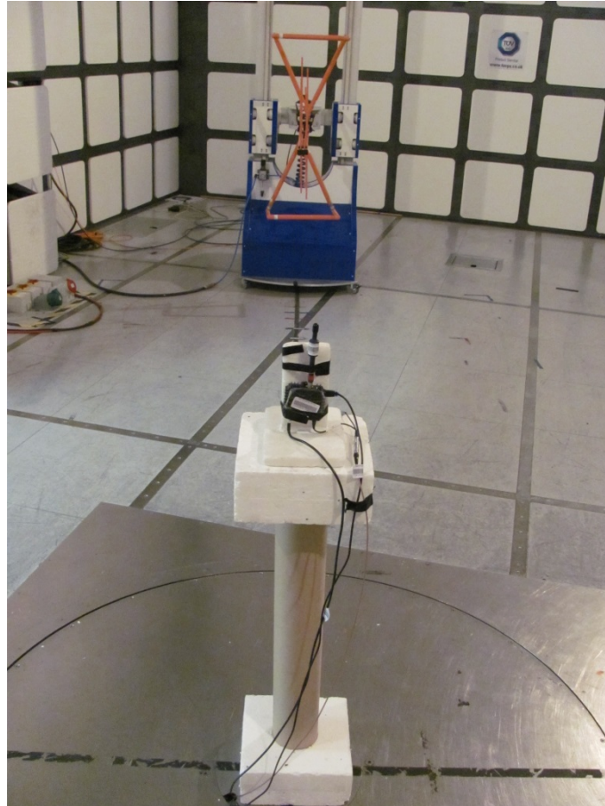
Radiated Emission 30 MHz to 1 GHz
