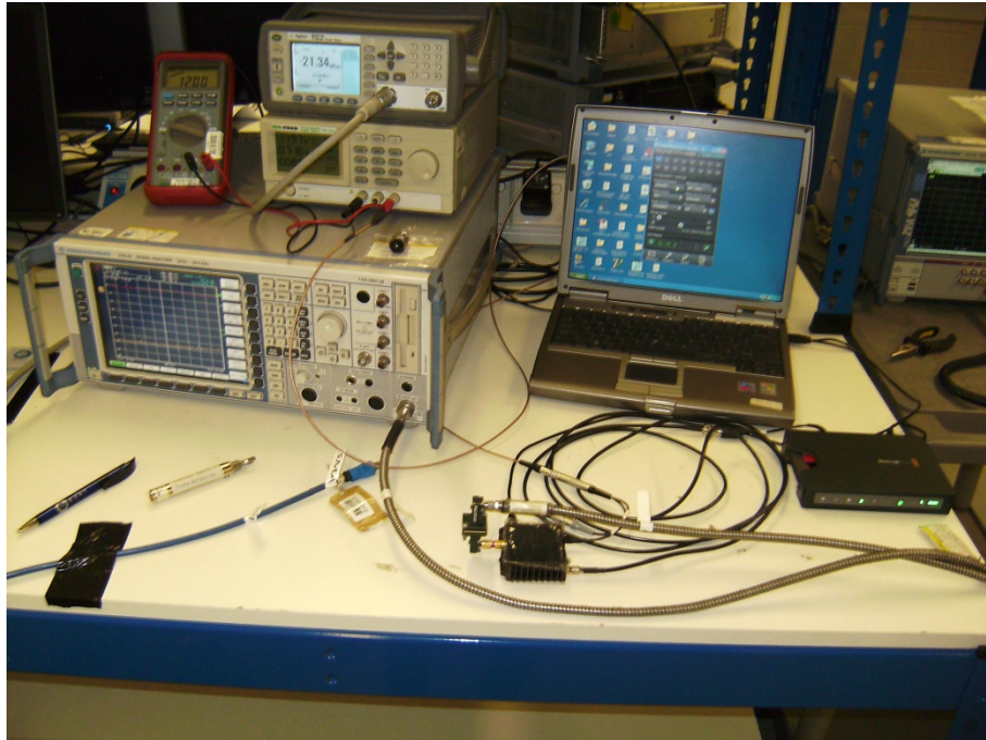
Conducted Set Up
