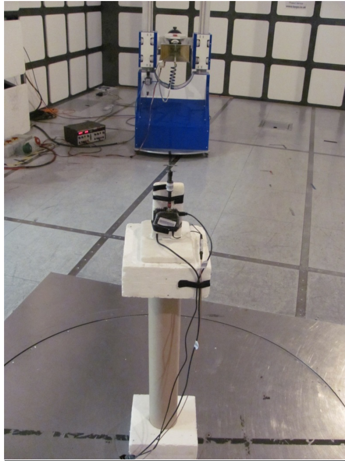
Radiated Emission 1 GHz to 18 GHz
