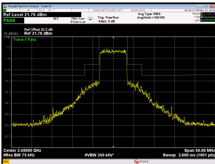
Figure 46 - Top Channel - Transmitter Mask - 7 MHz Bandwidth, Port A
