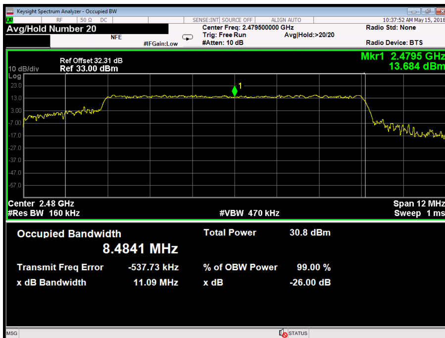
Figure 23 - Top Channel - Occupied Bandwidth - 8 MHz Bandwidth, Port A
