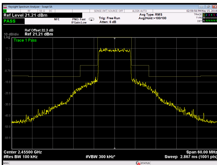
Figure 32 - Bottom Channel - Transmitter Mask - 10 MHz Bandwidth, Port A
