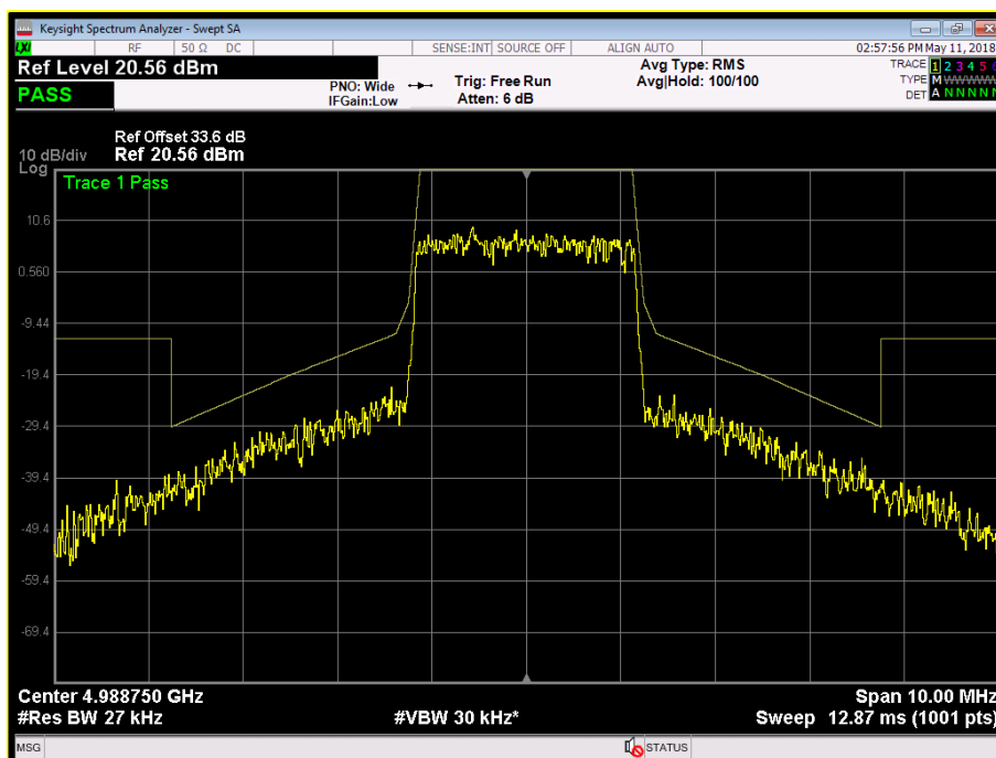
Figure 41 - Top Channel - Transmitter Mask - 2.5 MHz Bandwidth, Port A
