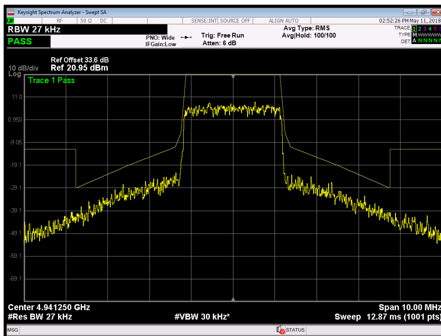
Figure 25 - Bottom Channel - Transmitter Mask - 2.5 MHz Bandwidth, Port A
