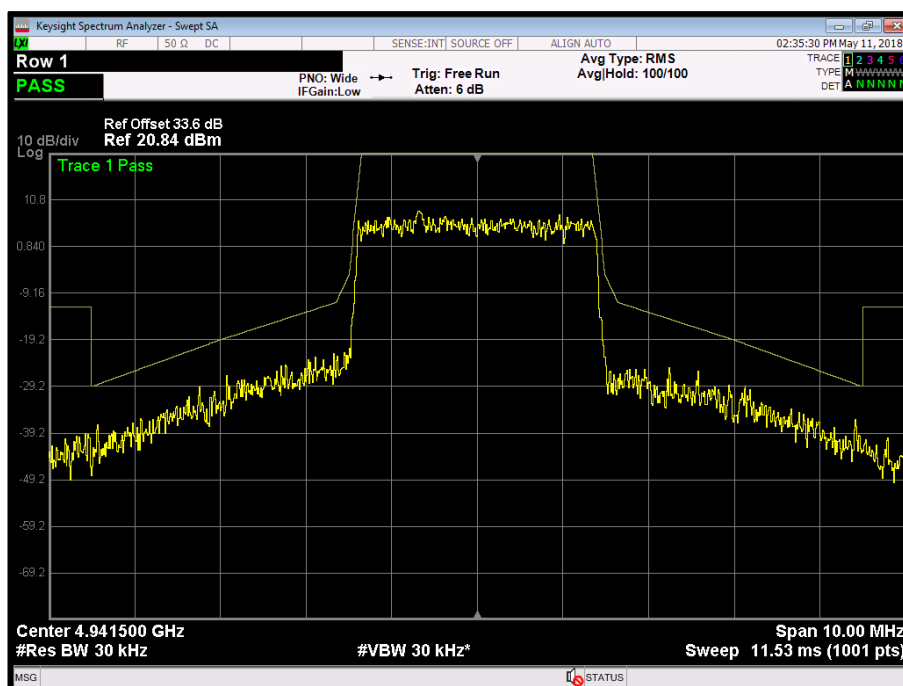
Figure 26 - Bottom Channel - Transmitter Mask - 3 MHz Bandwidth, Port A
