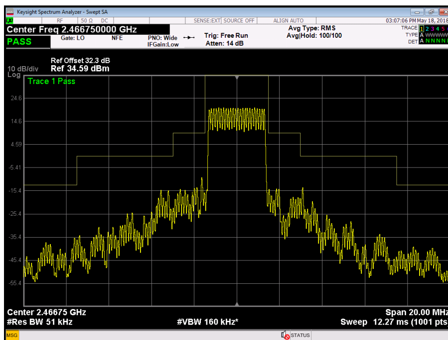
Figure 10 - Middle Channel - Transmitter Mask - 3 MHz Bandwidth, Port A
