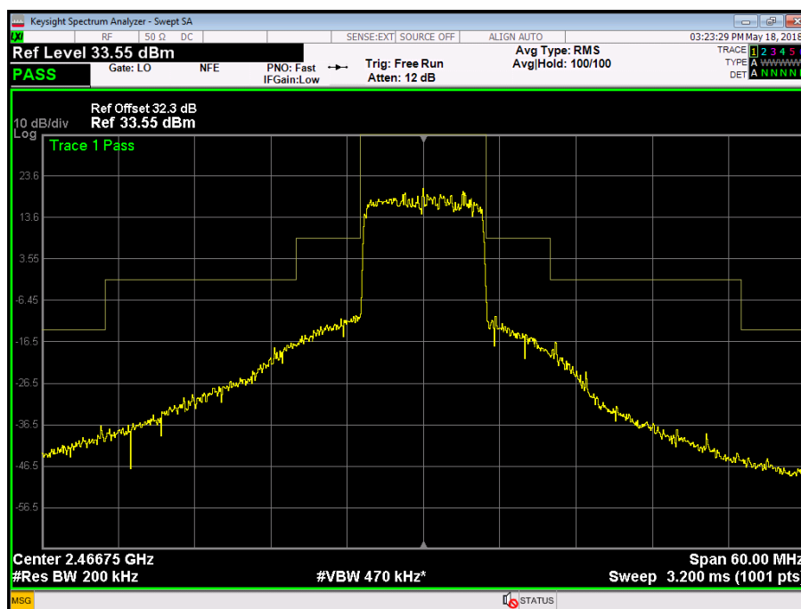
Figure 16 - Middle Channel - Transmitter Mask - 10 MHz Bandwidth, Port A
