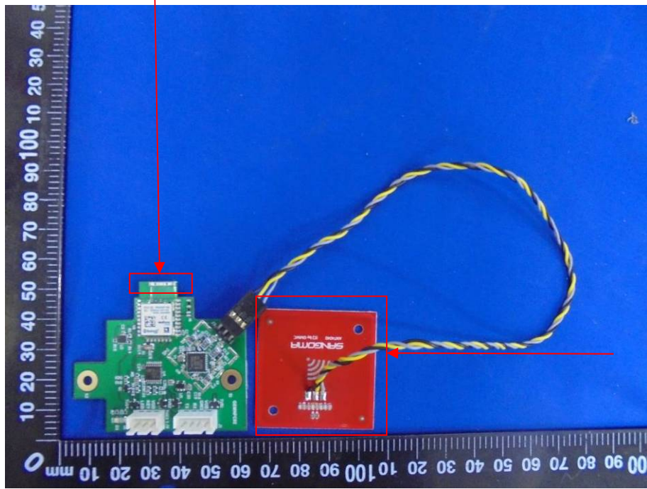
BT&ANT+ Antenna
