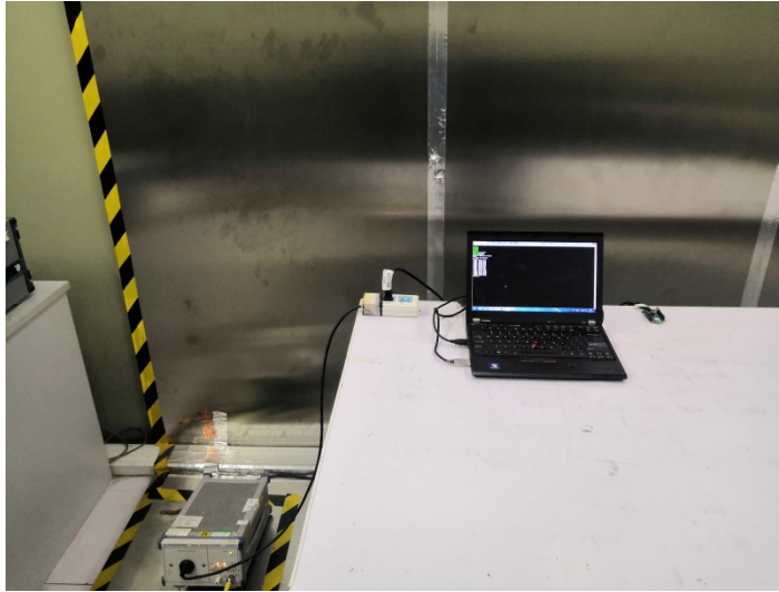
Conducted Emission
