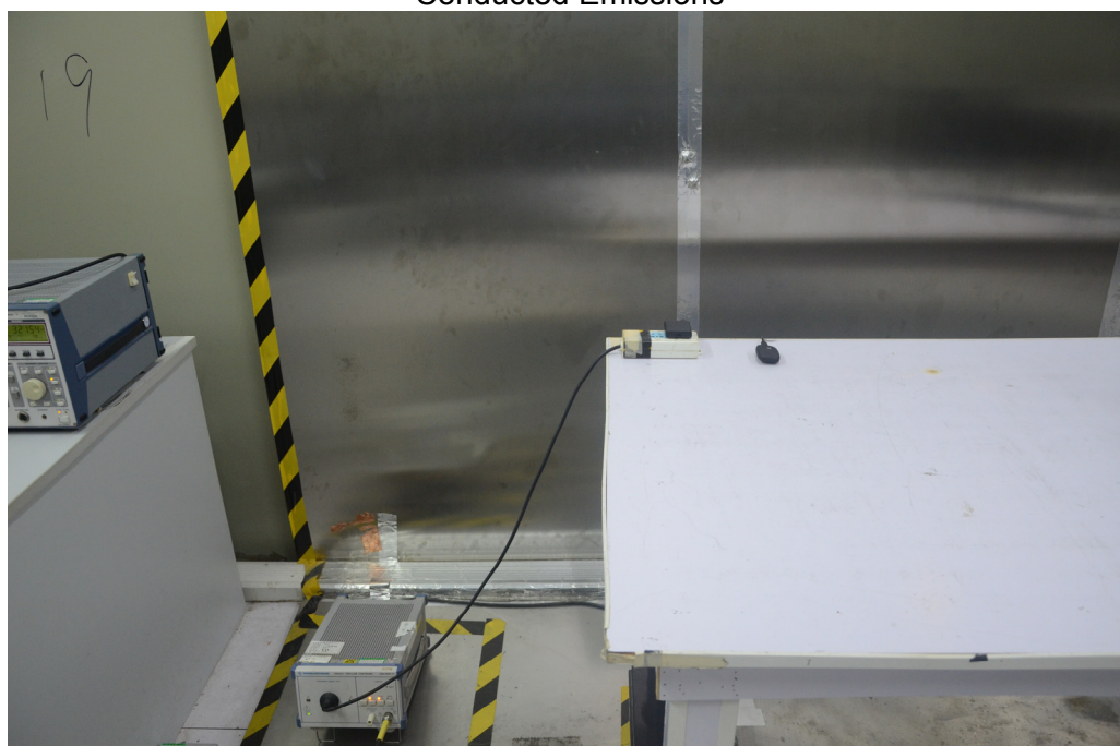
Conducted Emissions
