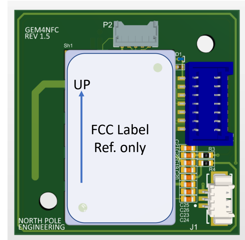
Fig 2 : Location and Orientation for FCC Label
