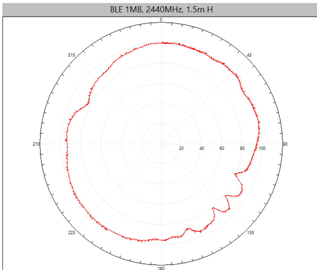
Figure 5 – Antenna Pattern, 1.5m Antenna height, 1.5m EUT Height
