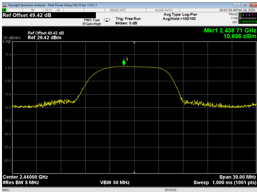
Figure 4 – Radiated Peak Power Measurement, BLE 1MB, Mid Channel Measurement corrections conversions are included in reference offset.
