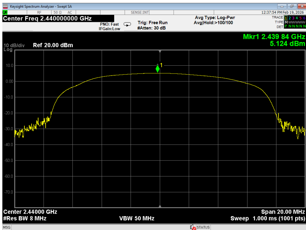
Figure 3 – Conducted Peak Power Measurement, BLE 1MB, Mid Channel
