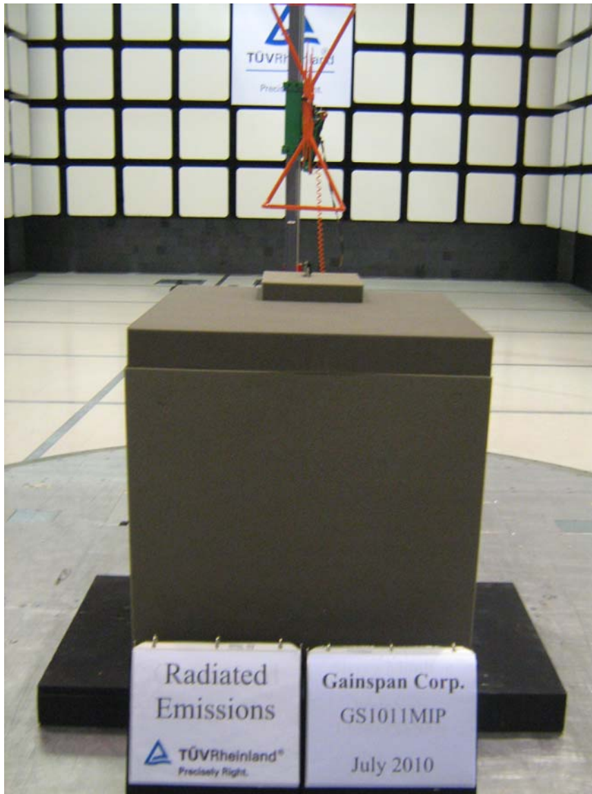
Figure 1: 30 MHz to 1000 MHz Radiated Emission Setup (Front View)
