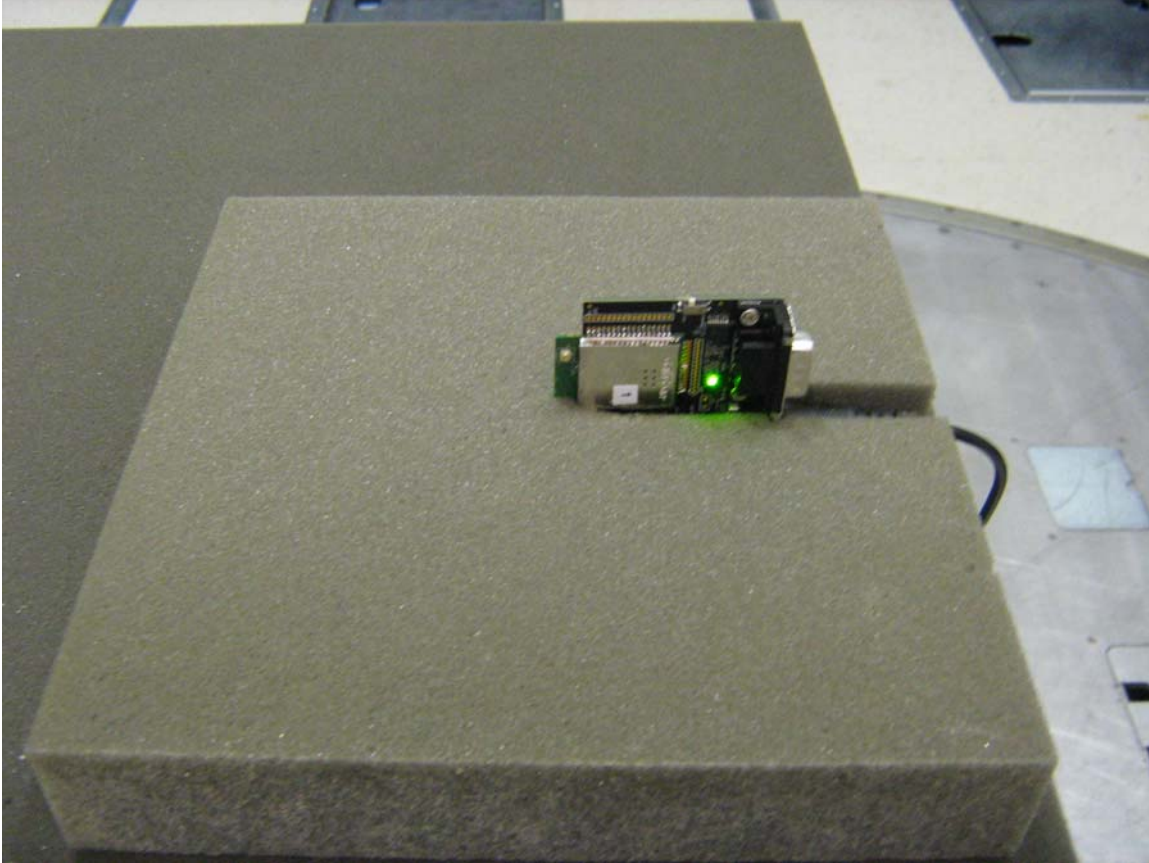
Figure 8: Radiated Emission Setup on Y-Axis
