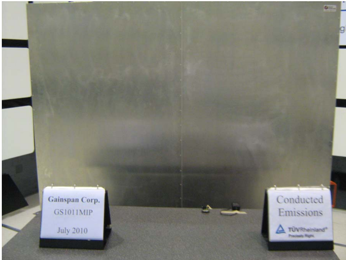
Figure 10: AC Conducted Emission (Front View)
