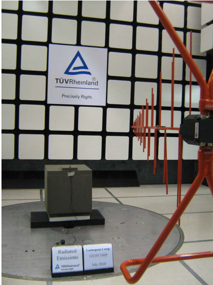
Figure 2: 30 MHz to 1000 MHz Radiated Emission Setup (Rear View)
