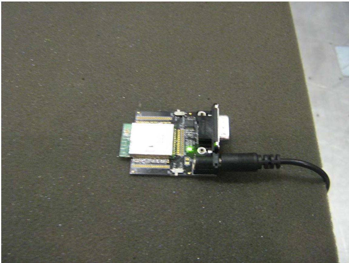
Figure 7: Radiated Emission Setup on X-Axis
