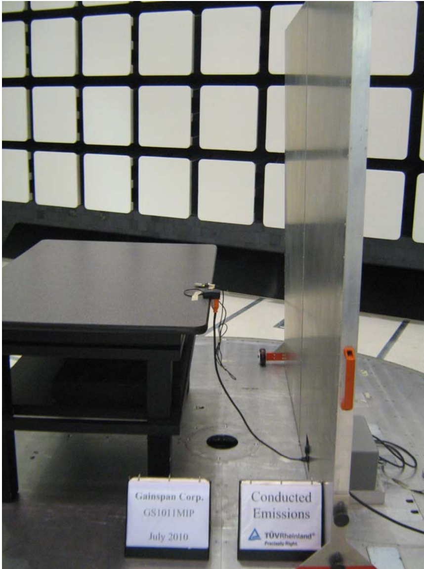
Figure 11: AC Conducted Emission (Side View)
