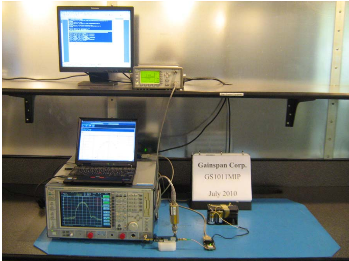
Figure 12: Conducted Test at RF Output Port for WiFi Module
