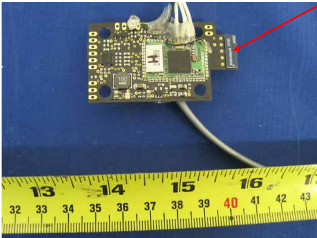
Bluetooth Radio Module- Antenna
