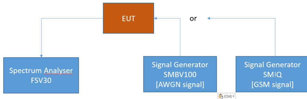
FCC Part 22/24/27/90 Industrial signal booster – Test Setup; RF Output Power / Gain
