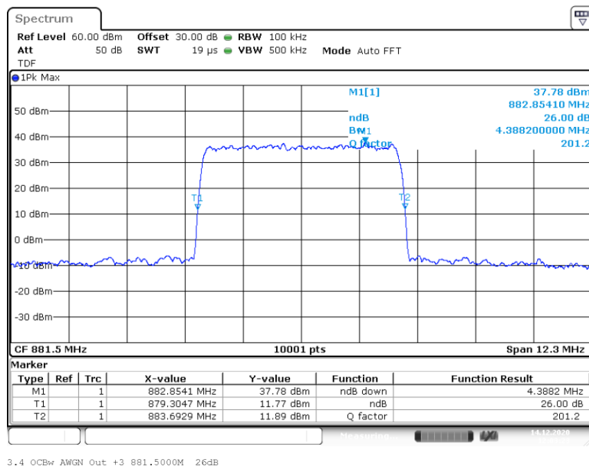
Output Signal
