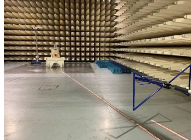
Radiated Measurement 30 MHz up to 1 GHz
