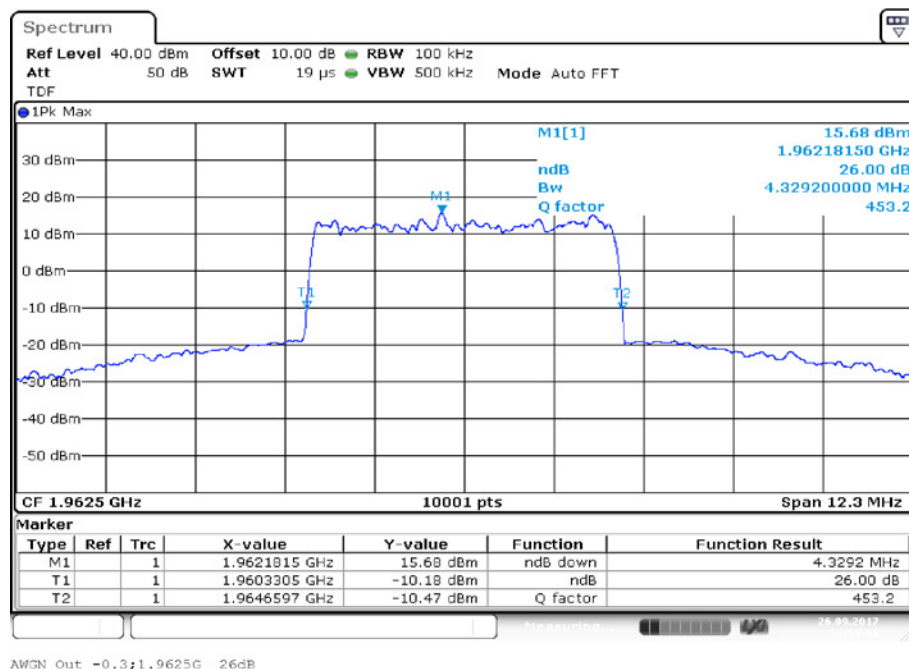
Output Signal
