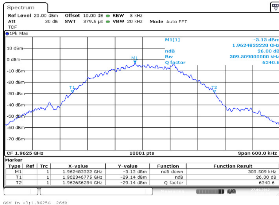
Input Signal
