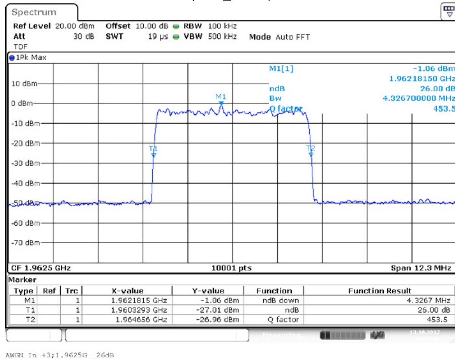
Input Signal
