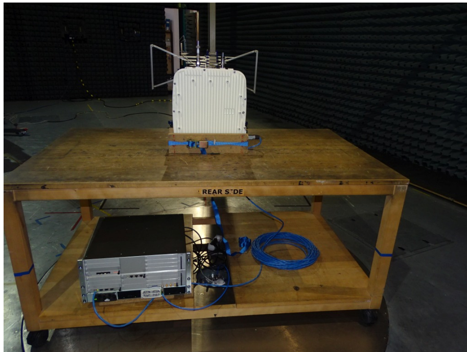
Photo 1: Test setup for radiated emissions measurements in semi-anechoic chamber (30 MHz to 1 GHz), rear side view with auxiliary equipment below table)
