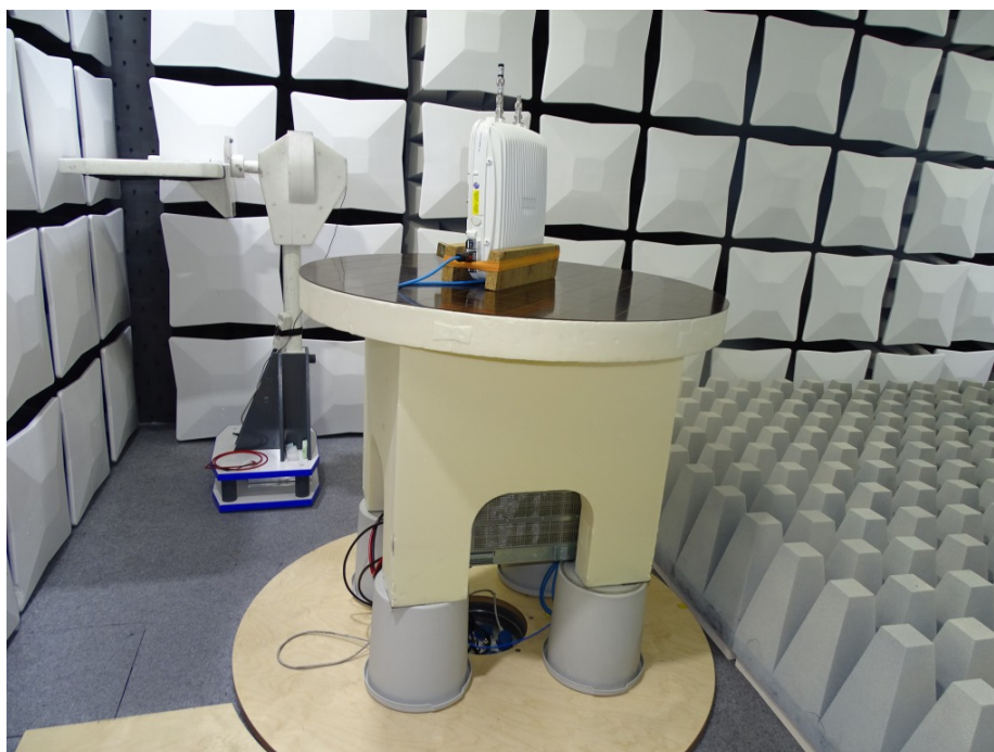
Photo 5: Test setup for radiated emissions measurements in fully-anechoic chamber (1 GHz to 27 GHz), front side view (with auxiliary equipment below table)
