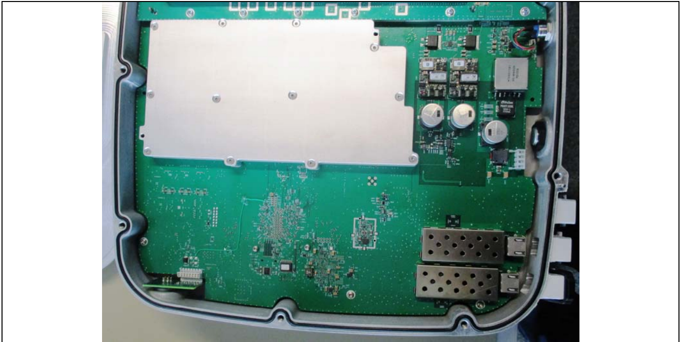
Main Board
