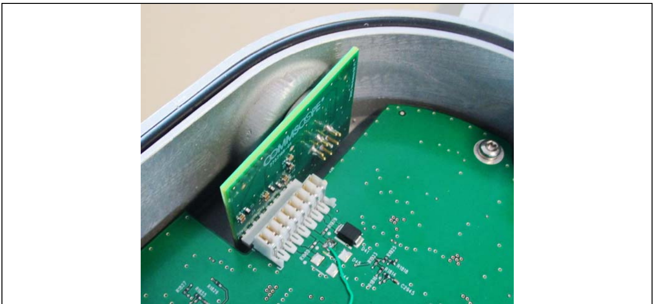
Fan Connector Board
