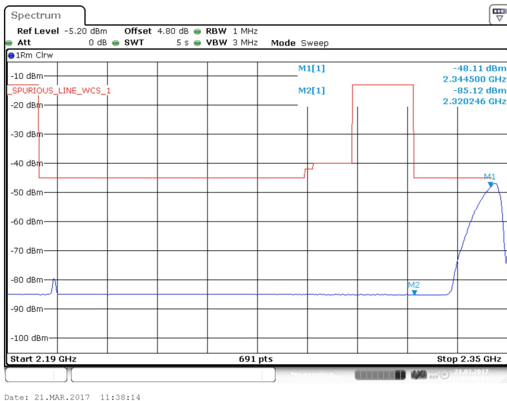
plot 7.3.1.1-#3 Spurious Emissions at Antenna Terminals: §27.53, §2.1051; Test results; Downlink; LTE; 2 x 5 MHz signal; 2.19 GHz – 2.35 GHz; carrier notched
