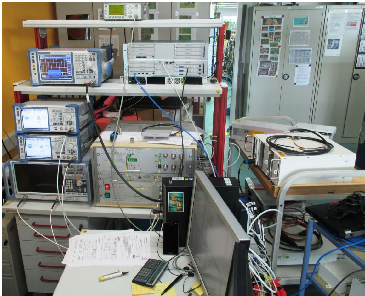
Measurement Equipment
