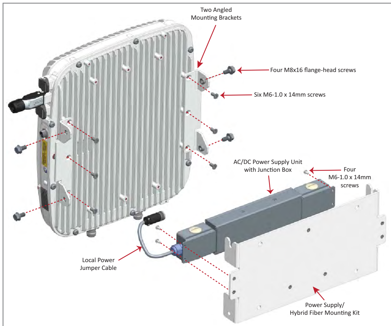
Figure 17. CAP L (No Fan Kit) with AC/DC Power Supply Kit (PN 7775087-xx) and Power Supply/Hybrid Fiber Mounting Kit (7774354-xx)
