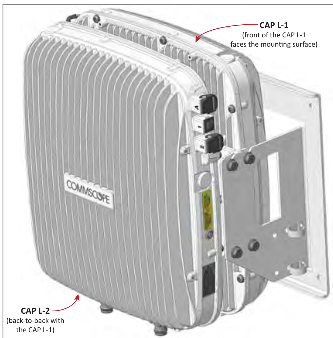
Figure 12. Two CAP Ls Back-to-Back in a Dual Mounting Bracket
