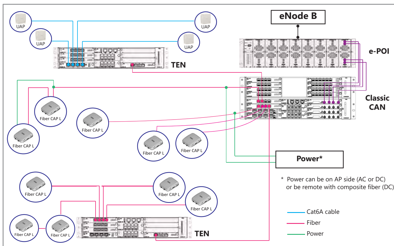
Figure 1. Fiber CAP L in an Era System
