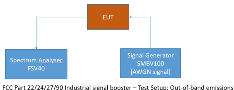
FCC Part 22/24/27/90 Industrial signal booster – Test Setup; Out-of-band emissions
