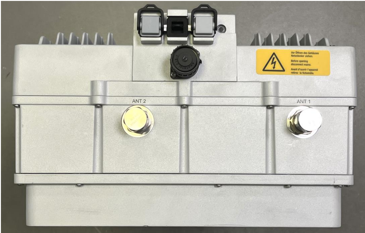
Fig. 6. Bottom View
