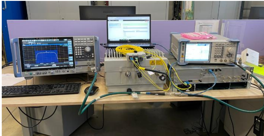
Figure-1: Antenna port testing set-up
