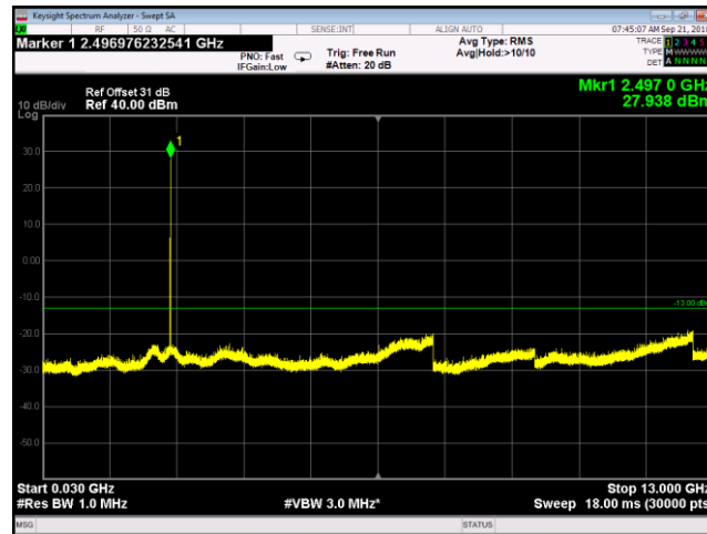
Plot 167. Spurious Emissions at Antenna Terminals, Band 41, 5 MHz, .03 -13 GHz, Low, Port 2
