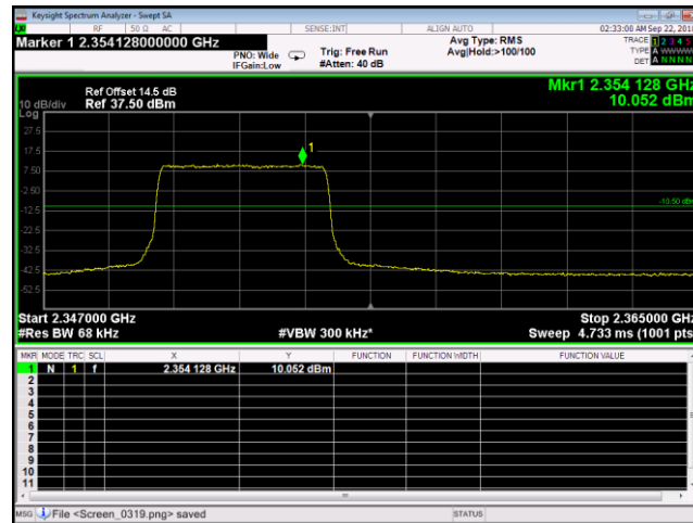
Plot 259. Intermodulation, WCS 2300, low channel, one signal, port 2, 5 MHz
