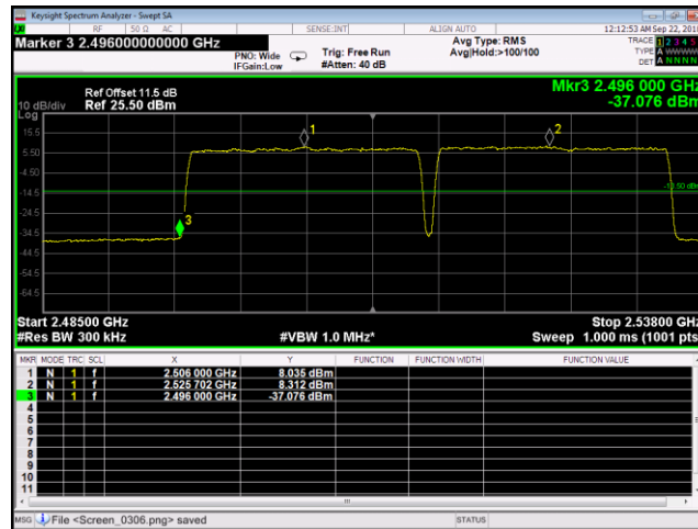
Plot 245. Antenna Terminals Band Edge, BRS 2500, low channel, two signal, port 1, 20 MHz
