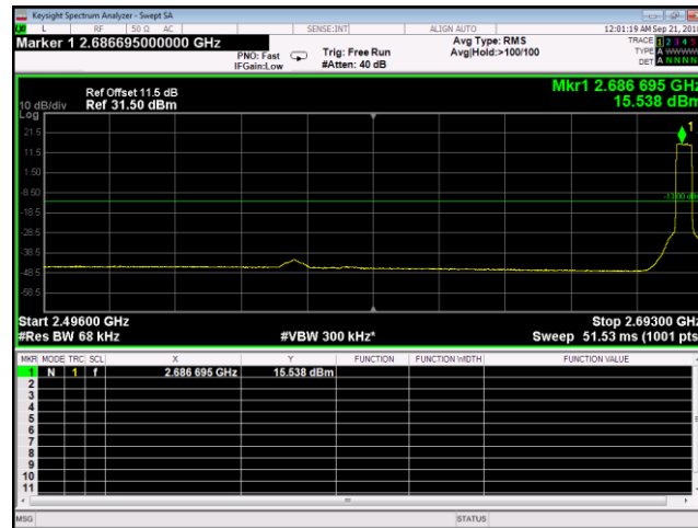
Plot 262. Intermodulation, BRS 2500, high channel, one signal, port 1, 5 MHz
