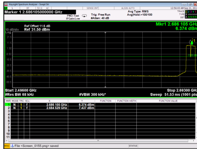
Plot 274. Intermodulation, BRS 2500, high channel, two signal, port 2, 5 MHz
