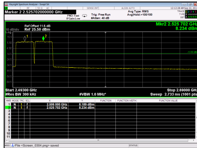
Plot 289. Intermodulation, BRS 2500, low channel, two signal, port 1, 20 MHz
