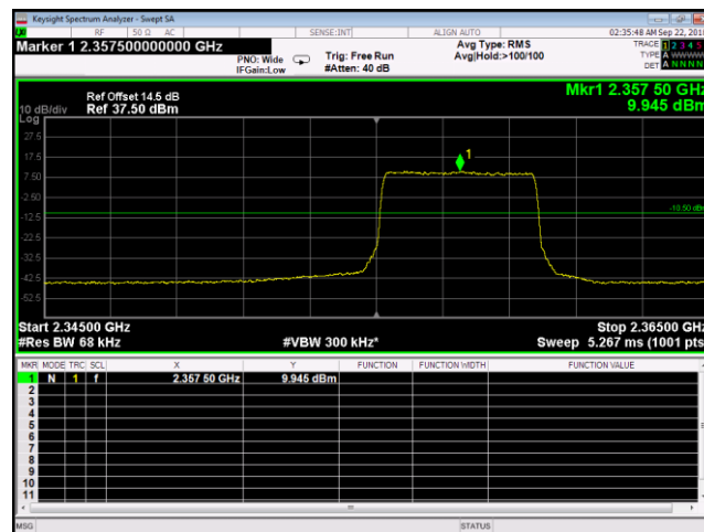
Plot 252. Intermodulation, WCS 2300, high channel, one signal, 1, 5 MHz
