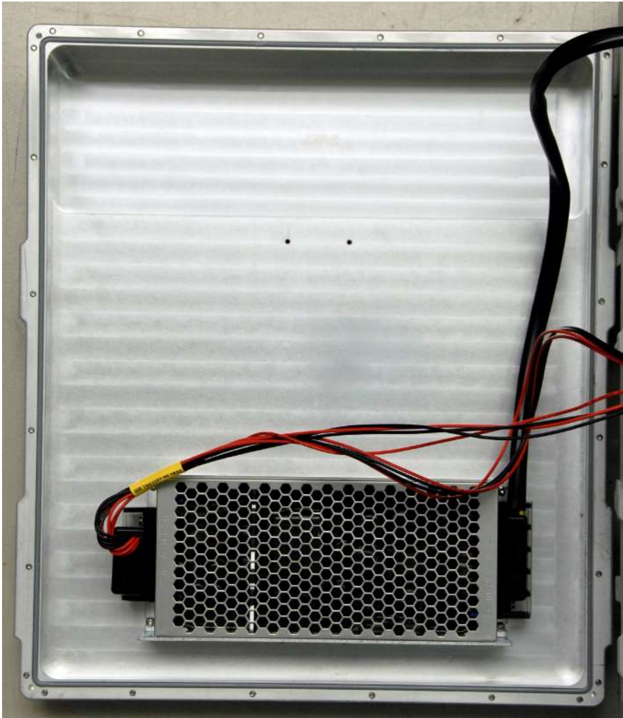
DC PSU inside
