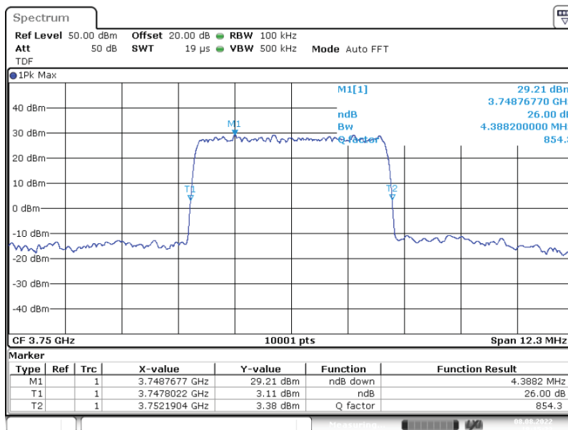
Output Signal
