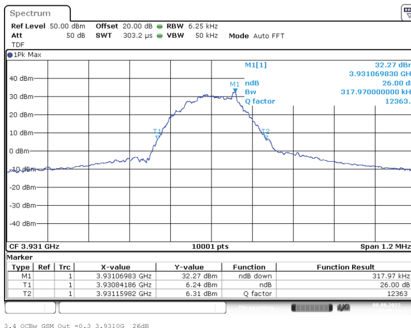
Output Signal
