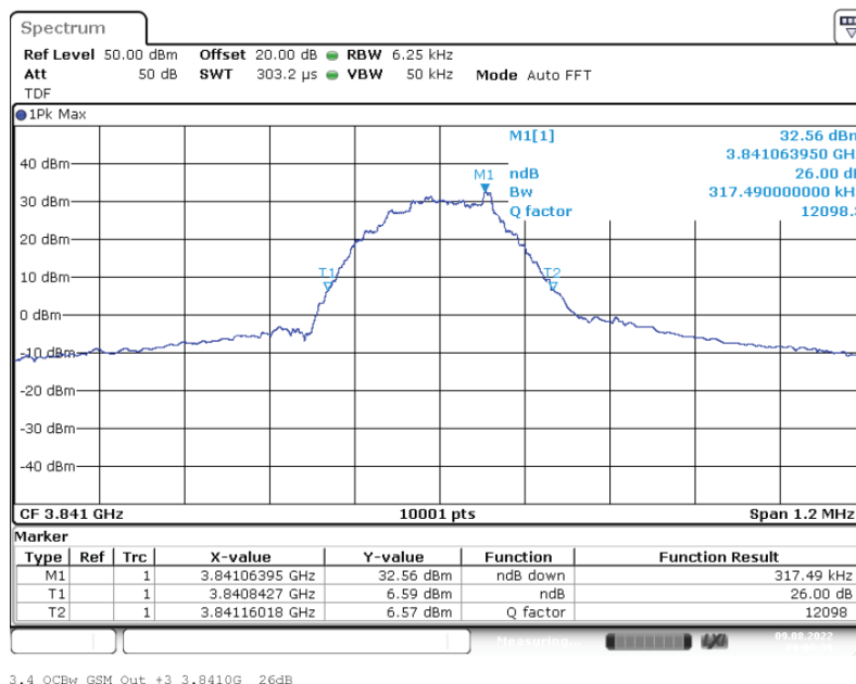
Output Signal
