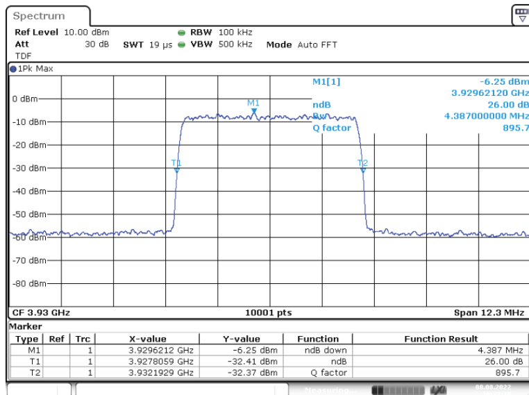
Input Signal
