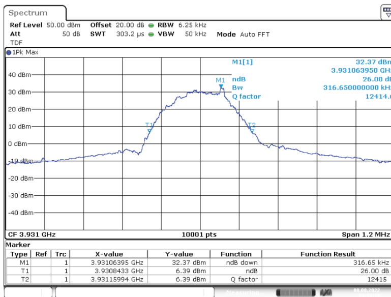
Output Signal
