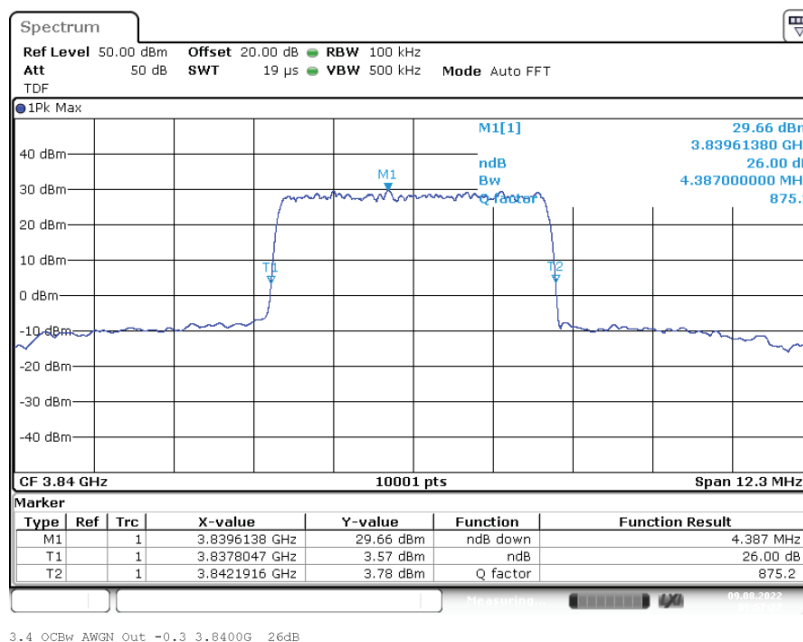
Output Signal
