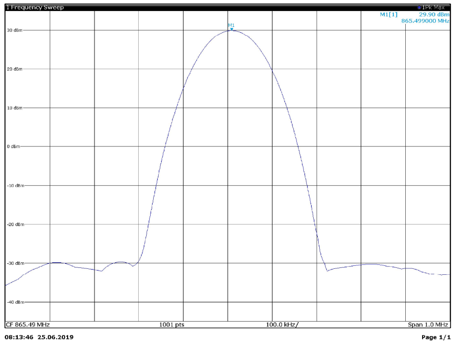
Output spectral plot with input at AGC threshold + 1 dB with CW signal at 865.5 MHz
