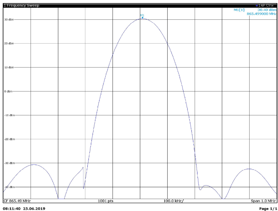
Output spectral plot with input at AGC threshold with 11K0F3E signal at 865.5 MHz
