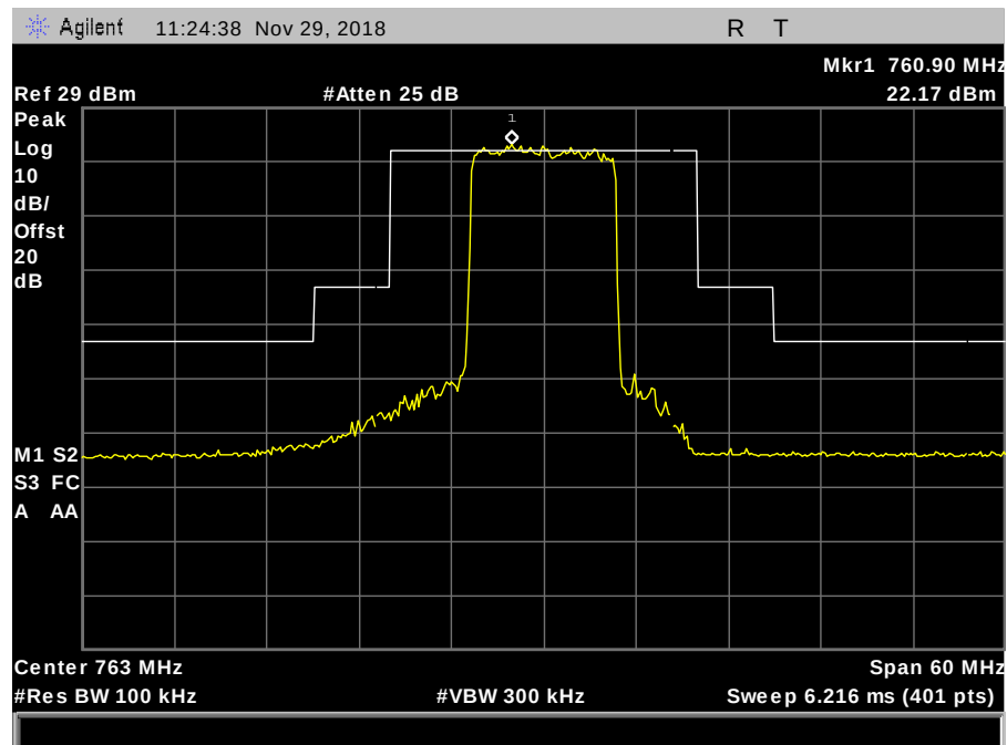
Plot 110. Emissions Mask, FCC90R, 763 MHz, Channel 10 MHz
