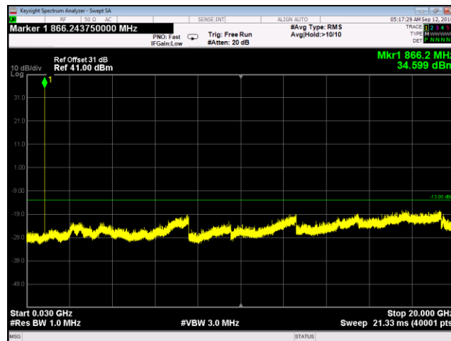
Plot 100. Spurious Emissions at Antenna Terminals, CDMA800, 862 - 869 MHz, Mid
