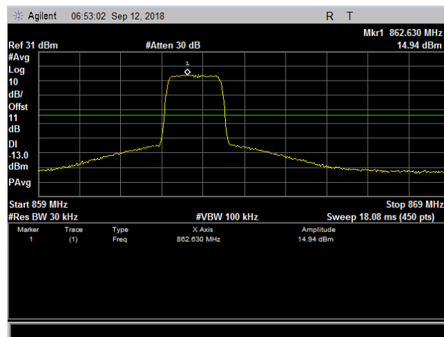
Plot 62. Intermodulation, CDMA SMR800, Low Channel, One Signal Intermodulation
