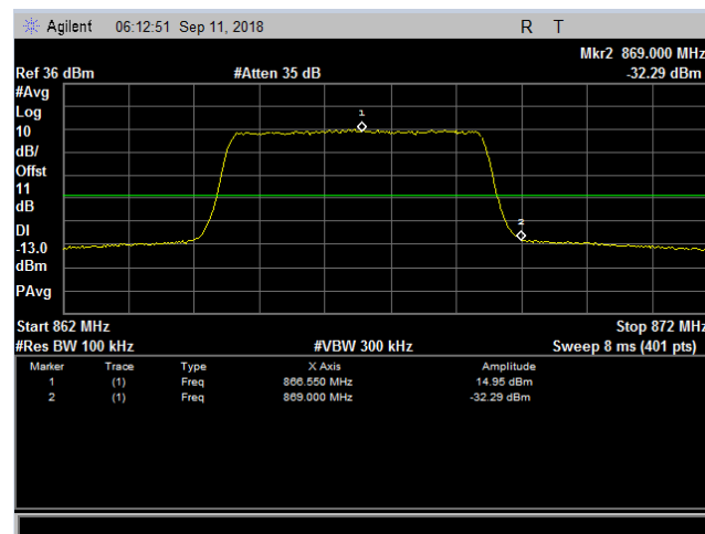
Plot 105. Band-Edge Channel Power, SMR800, High Channel, One Signal Band Edge
