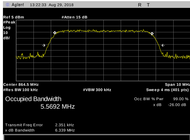
Plot 39. Occupied Bandwidth, SMR800, SG, Low, 862 – 869 MHz
