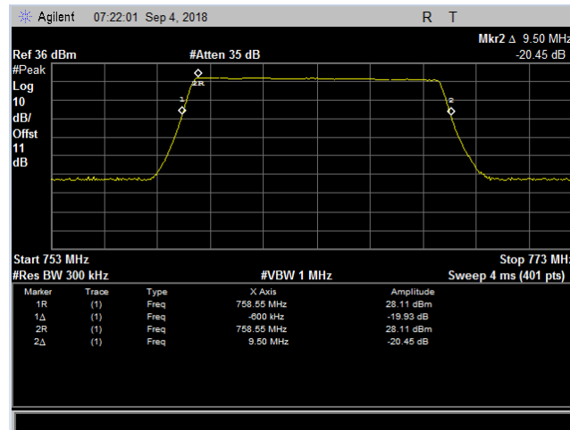
Plot 107. Filter Response, 758 – 768 MHz, Out of Band Rejection, LMR 750, band 14
