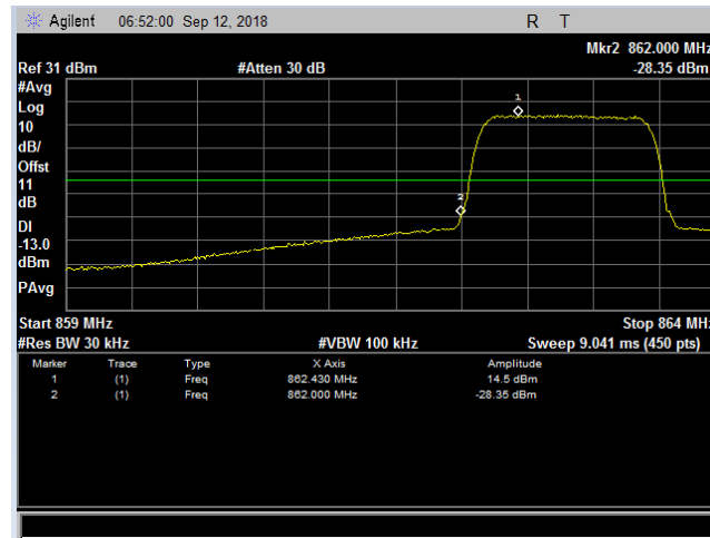
Plot 104. Band-Edge Channel Power, SMR800, Low Channel, One Signal Band Edge
