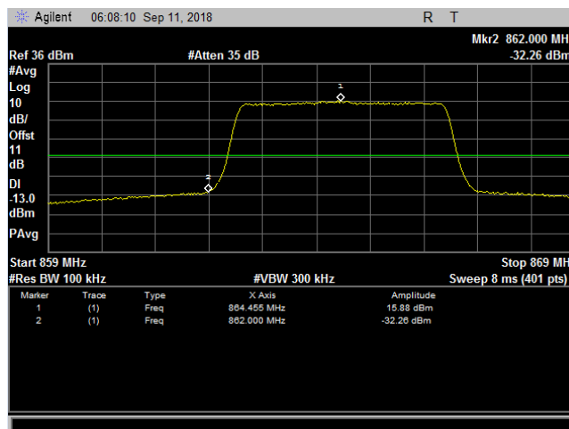
Plot 106. Band-Edge Channel Power, SMR800, Low Channel, One Signal Band Edge
