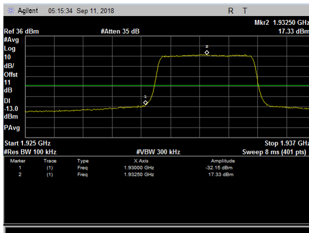
Plot 179. Band-Edge Channel Power, WCDMA 1900, Low Channel, One Signal Band Edge
