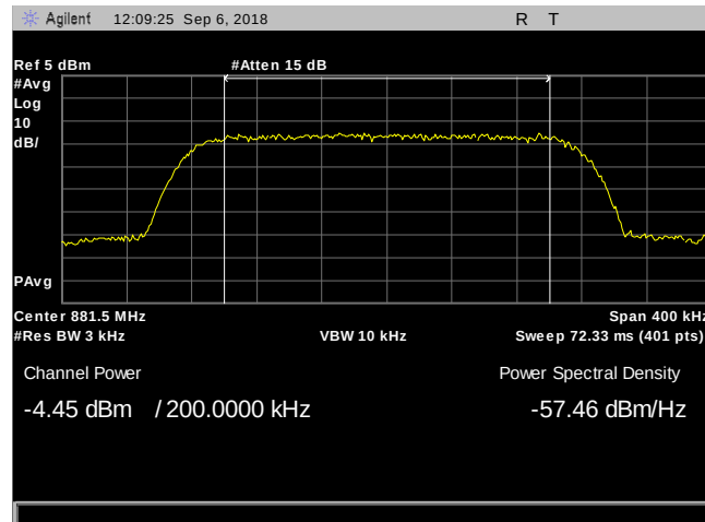
Plot 24. Output Power, CEL850, 869 – 894 MHz, Mid, AGC
