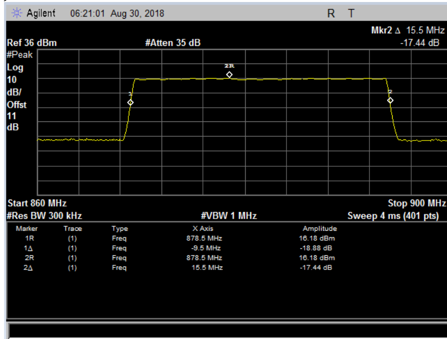
Plot 221. Filter Response, 869 – 894 MHz, Band of Rejection Cell 850
