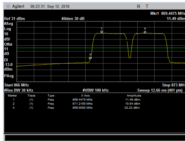
Plot 156. Band-Edge Channel Power, CDMA Cell 850, Low Channel, Two Signal Band Edge
