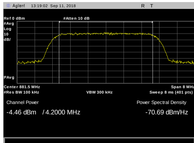
Plot 36. Output Power, WCDMA850, SG, 869 - 894 MHz, Mid
