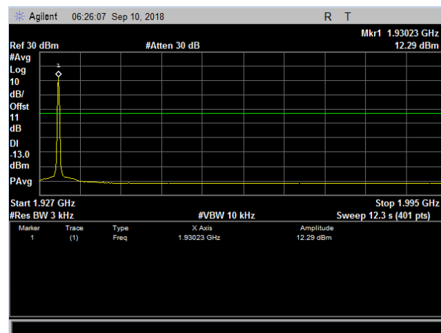
Plot 205. Intermodulation, GSM 1900, Low Channel, One Signal Intermodulation
