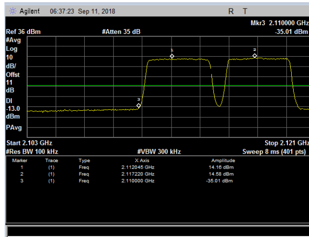
Plot 184. Band-Edge Channel Power, WCDMA AWS 1700, Low Channel, Two Signal Band Edge
