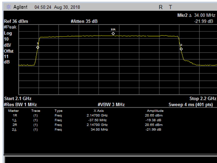
Plot 223. Filter Response, 2110 – 2180 MHz, Out of Band Rejection, AWS Band
