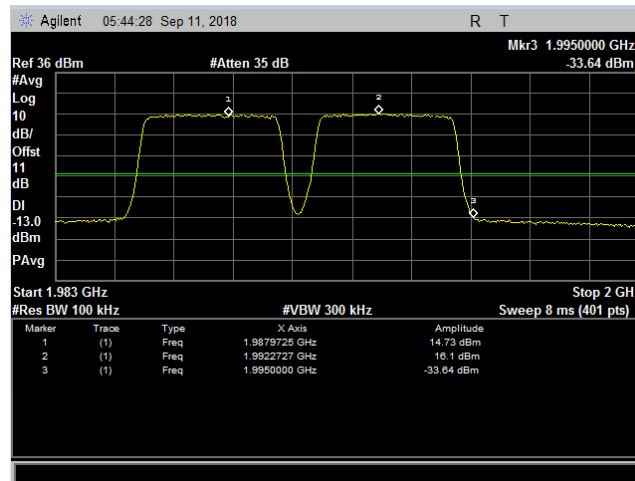
Plot 178. Band-Edge Channel Power, WCDMA 1900, High Channel, Two Signal Band Edge
