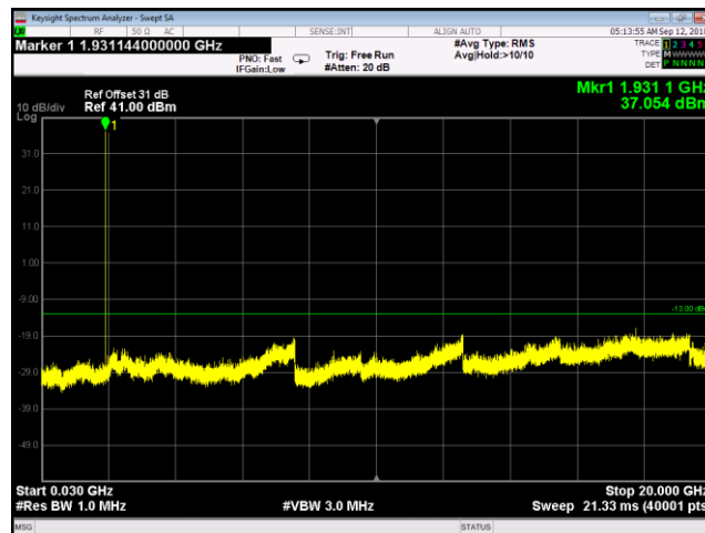
Plot 133. Spurious Emissions at Antenna Terminals, CDMA1900, 1930 - 1995 MHz, Low
