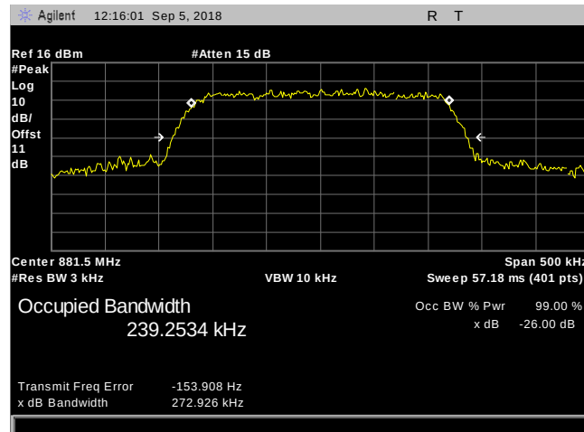
Plot 72. Occupied Bandwidth, GSM850, SG, 869.2 - 893.8 MHz, Mid
