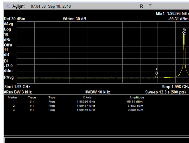
Plot 204. Intermodulation, GSM 1900, High Channel, Two Signal Intermodulation
