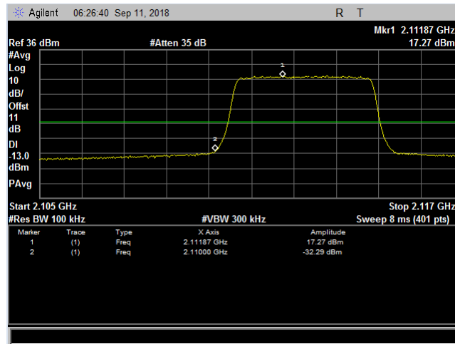
Plot 183. Band-Edge Channel Power, WCDMA AWS 1700, Low Channel, One Signal Band Edge
