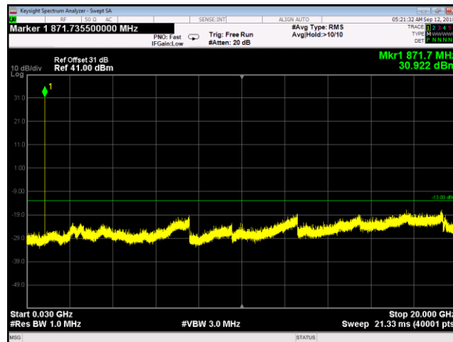
Plot 145. Spurious Emissions at Antenna Terminals, WCDMA850, 824 - 869 MHz, Low
