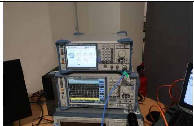
Conducted Mesurements
