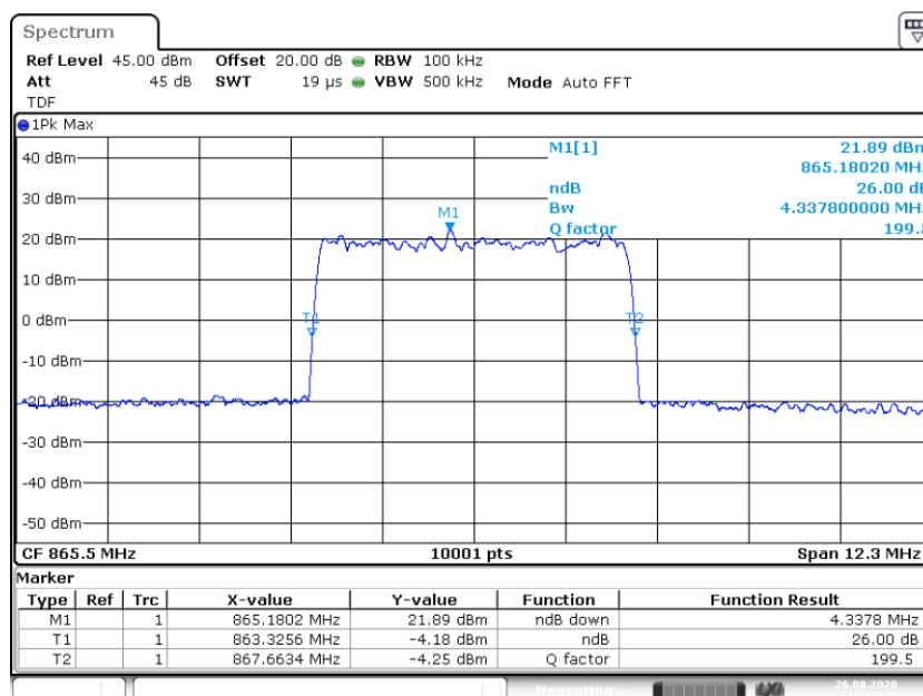
Output Signal
