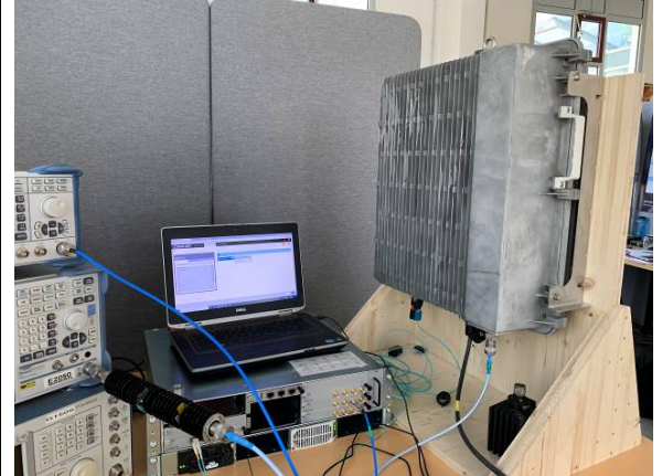
Conducted Mesurements
