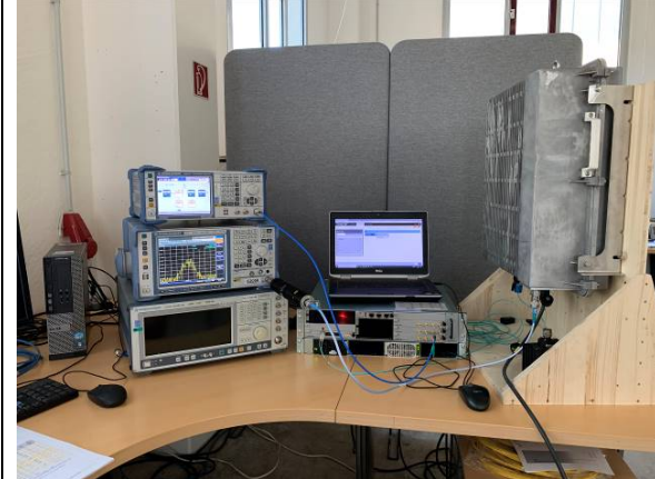
Conducted Mesaruements
