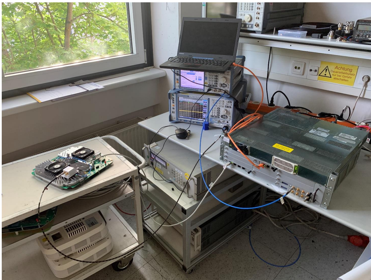
Photograph: Setup of conducted measurements.
