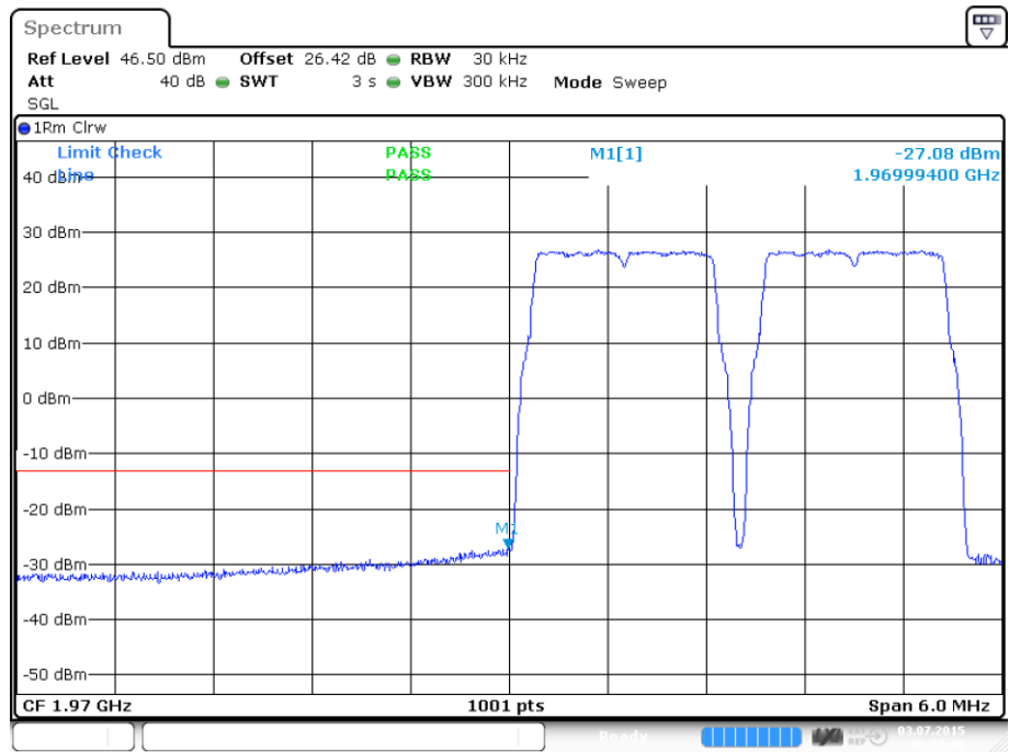
plot 8.3.1.3-#1 Intermodulation: §24.238, §2.1051; Test results; Downlink; LTE Lower Band Edge
