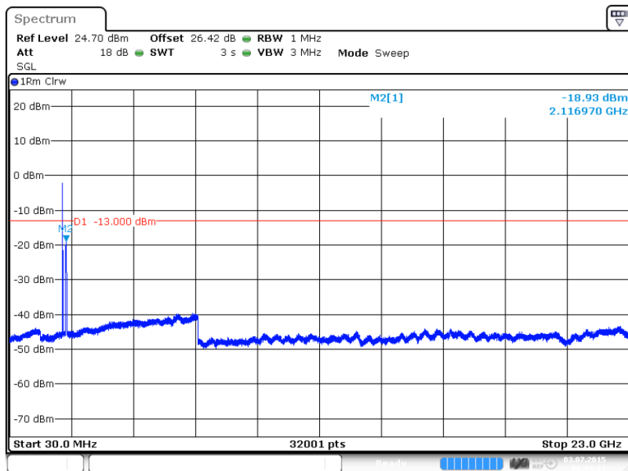
plot 7.3.1.3-#1 Spurious Emissions at Antenna Terminals: §24.238, §2.1051; Test results; Downlink; LTE; carrier (1980 MHz) notched
