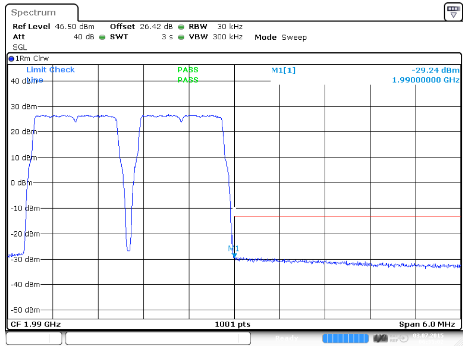
plot 8.3.1.3-#2 Intermodulation: §24.238, §2.1051; Test results; Downlink; LTE Upper Band Edge
