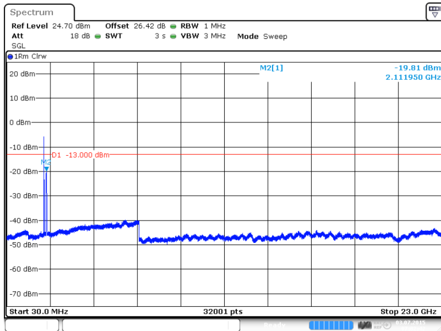
plot 7.3.1.2-#1 Spurious Emissions at Antenna Terminals: §24.238, §2.1051; Test results; Downlink; WCDMA; carrier (1980 MHz) notched
