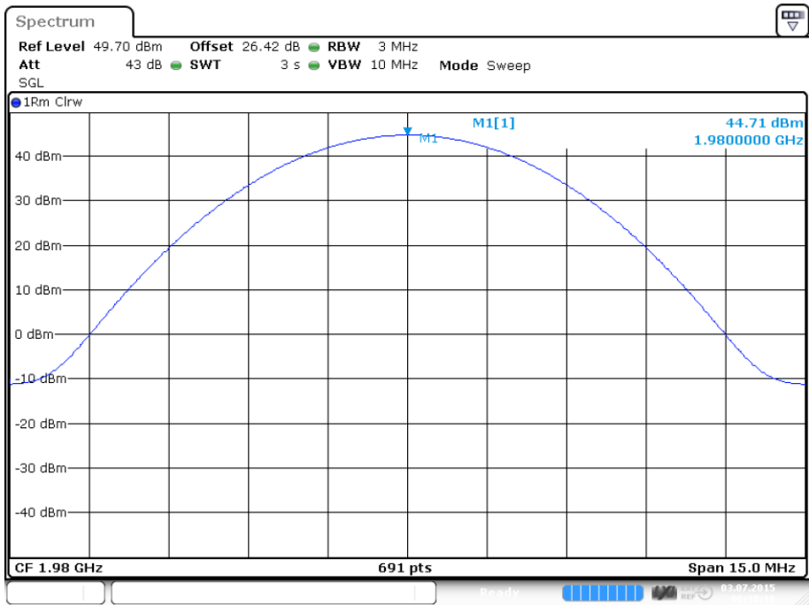
plot 5.3.1.1-#1 RF Power Out: §24.232, §2.1046; Test Results; Downlink; CDMA Middle
