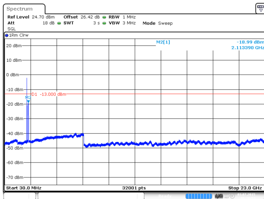
plot 7.3.1.1-#1 Spurious Emissions at Antenna Terminals: §24.238, §2.1051; Test results; Downlink; CDMA; carrier (1980 MHz) notched
